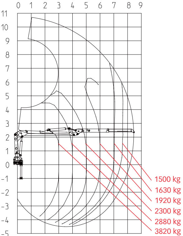
Load diagram JONSERED 1188S84i
