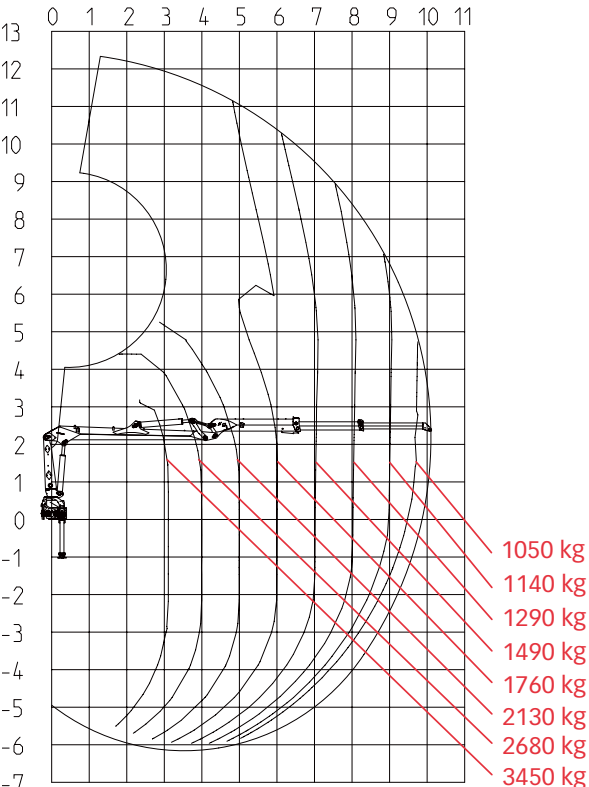
Load diagram JONSERED 1188S101i
