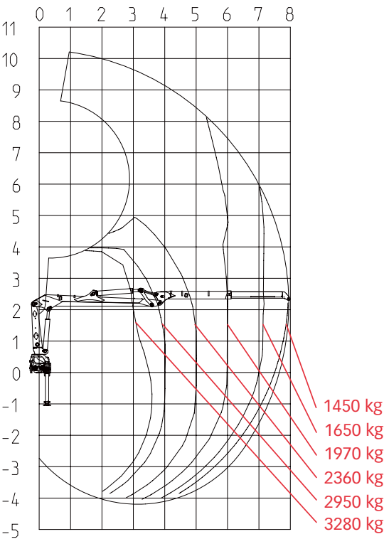
Load diagram JONSERED 1188S79i
